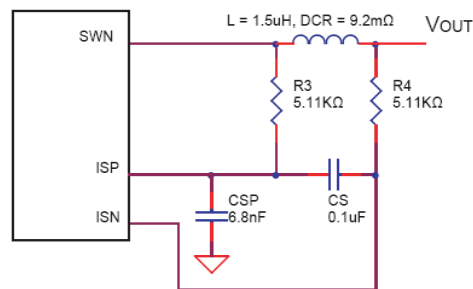
Fig. 16: Over Current Detection Circuit
