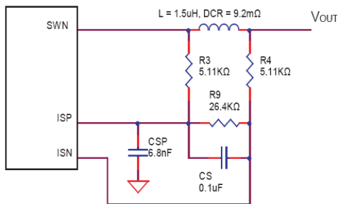
Fig. 17: Over Current Detection Circuit for I_{MAX} > 60mV/DCR
