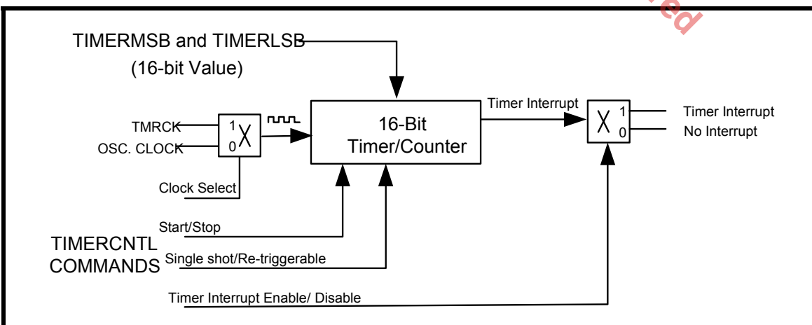
FIGURE 14. TIMER/COUNTER CIRCUIT
