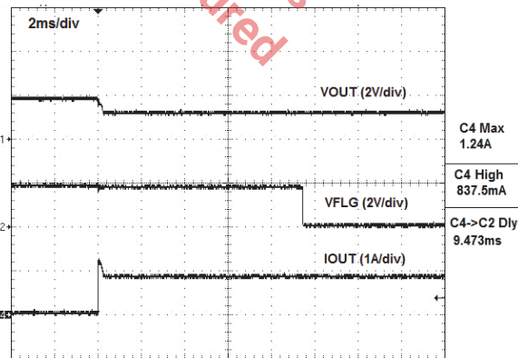
Fig. 27: Current Limit Operation (XRP2528): VIN=1.8V, Rload = 1.5Ω, USB2.0
