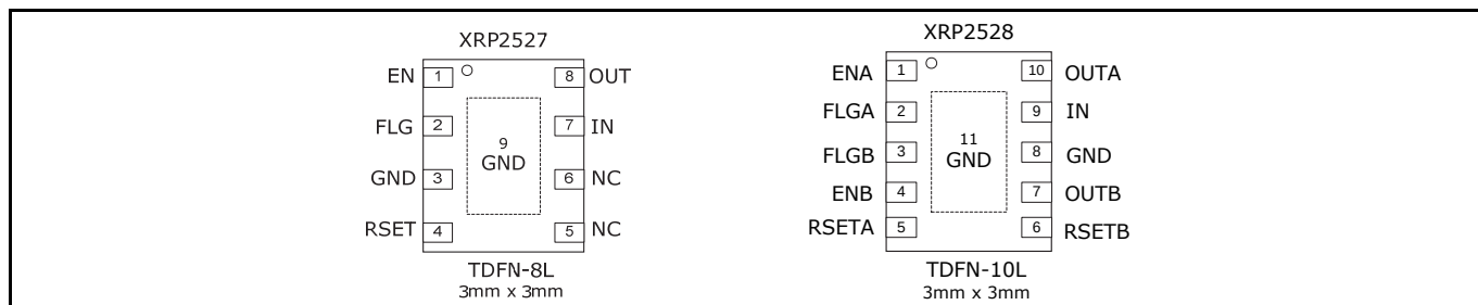
Fig. 3: XRP2527/28 Pin Assignment
