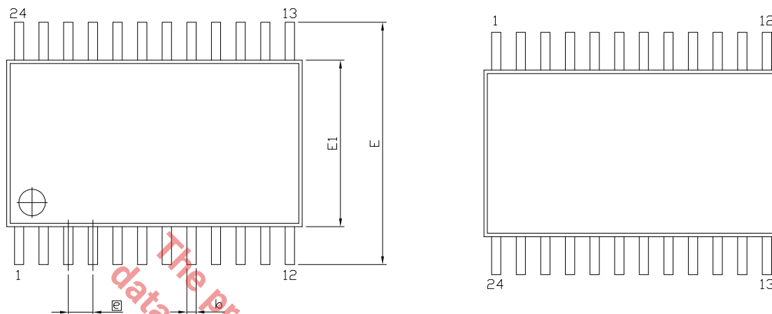
TOP VIEW
