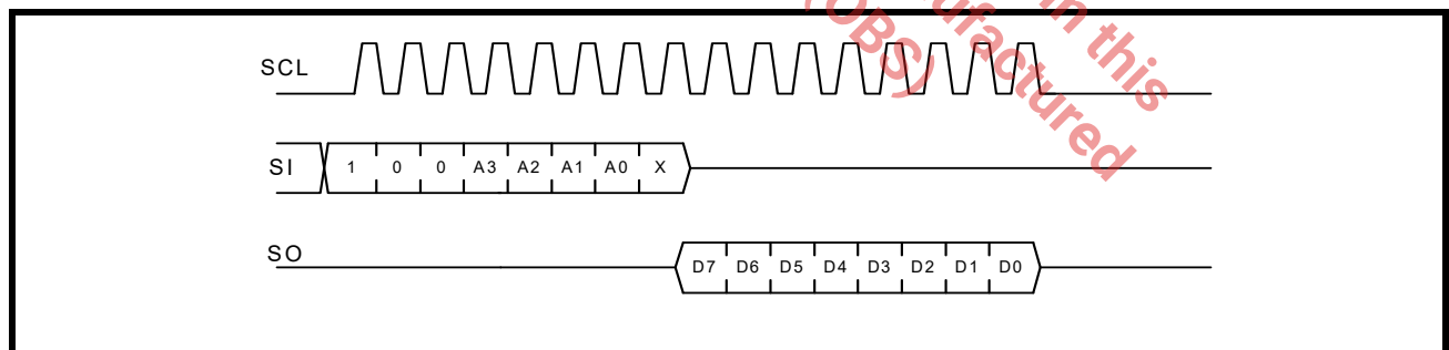
FIGURE 4. SPI READ
