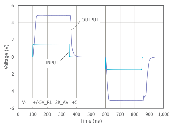
Figure 5: Overdrive Recovery
