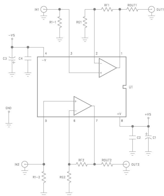
Figure 13. CEB006 & CEB010 Schematic
