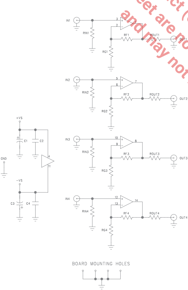
Figure 10. CEB018 Schematic
