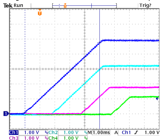
Figure 9: Sequential Start-up
