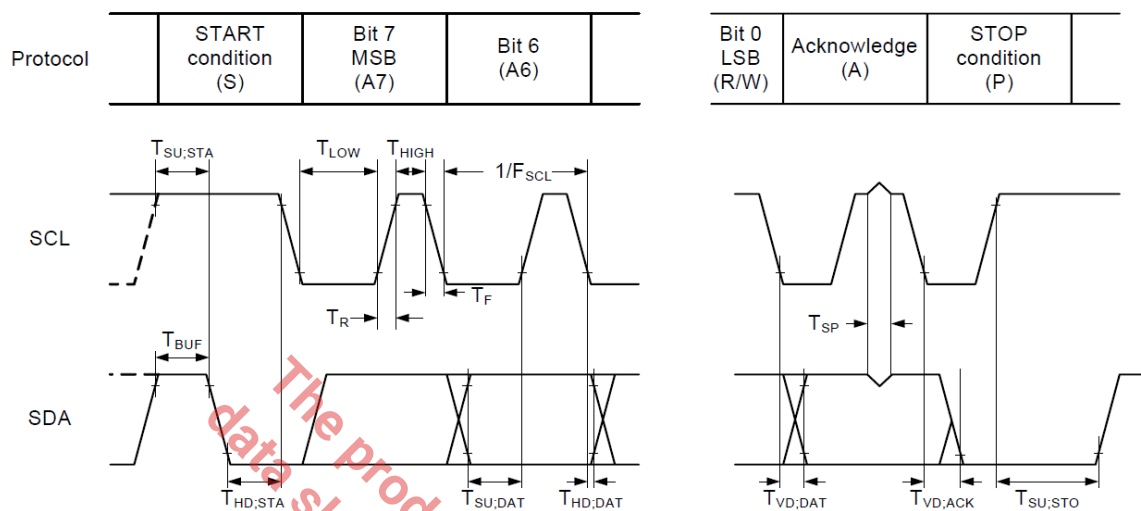
Figure 3: I²C Bus Timing Diagram
