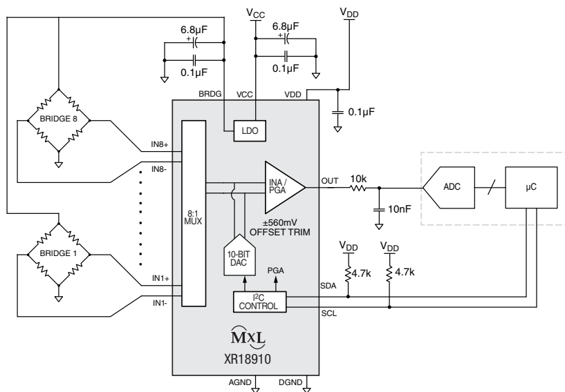
Figure 1. Typical Application
