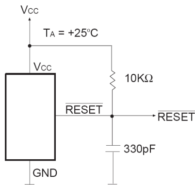
Fig. 11: SP705/707 RESET Response Time Circuit
