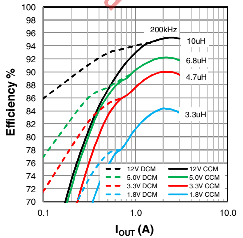
Figure 24: XR76203-Q Efficiency, V_{IN} = 24\text{V}
