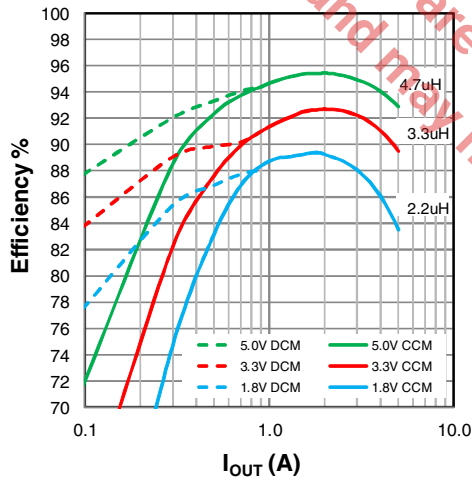
Figure 21: XR76205-Q Efficiency, V_{IN} = 12\text{V}
