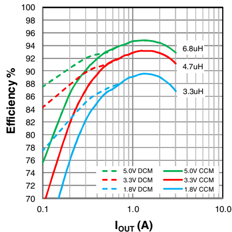
Figure 23: XR76203-Q Efficiency, V_{IN} = 12\text{V}
