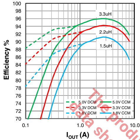
Figure 19: XR76208-Q Efficiency, V_{IN} = 12\text{V}
