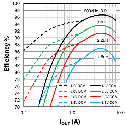
Figure 20: XR76208-Q Efficiency, V_{IN} = 24\text{V}
