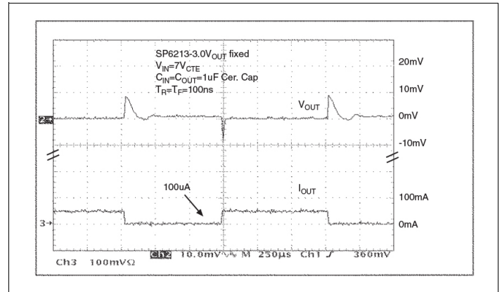
Figure 30: Load Transient Response ( V_{IN} = 7V )
