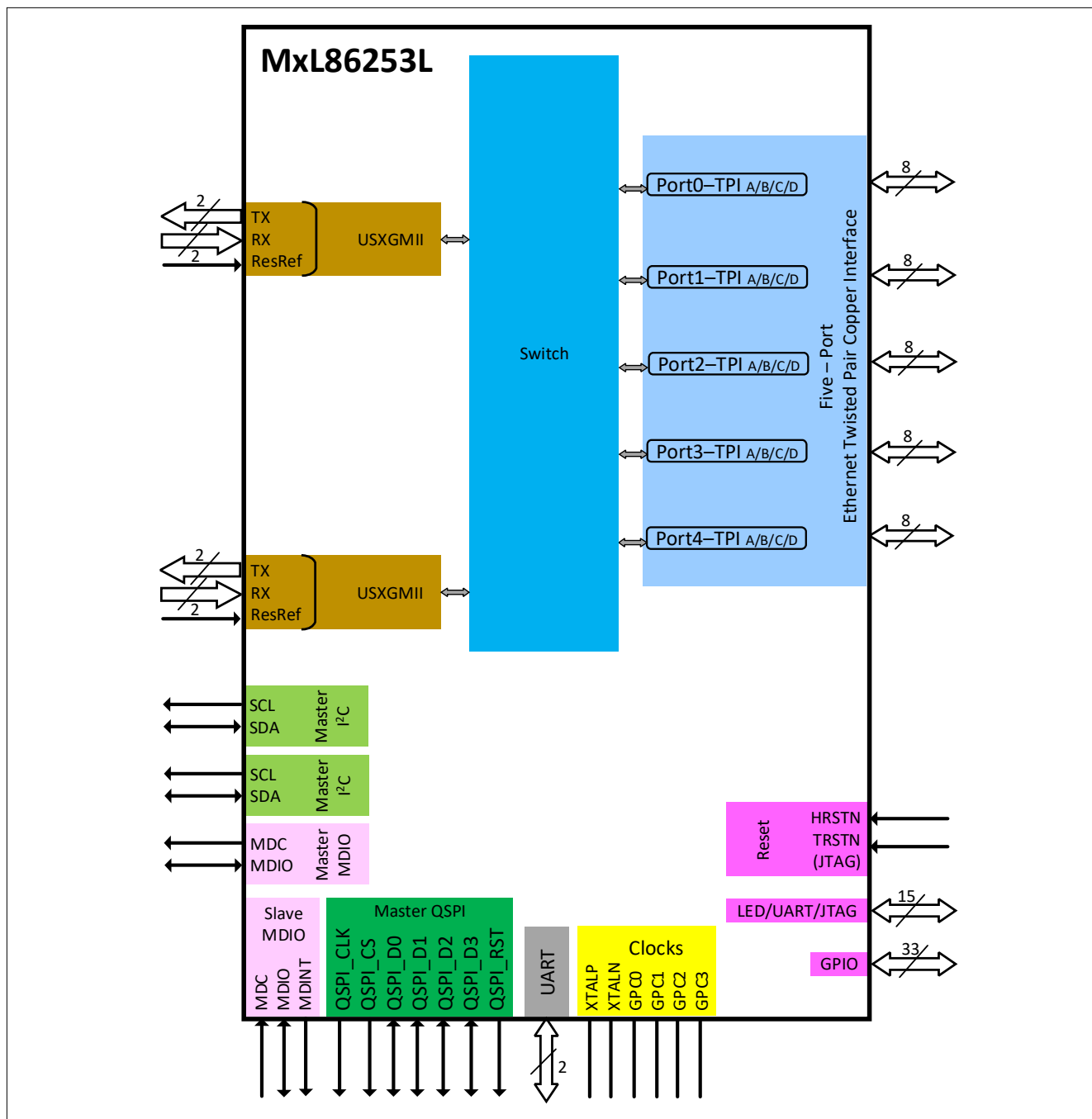
Figure 1 MxL86253L Block Diagram
