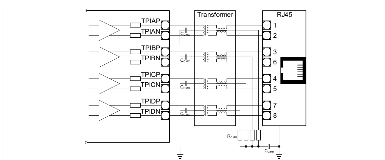
Figure 6 Twisted-Pair Interface of MxL86253L Including Transformer and RJ45 Plug
