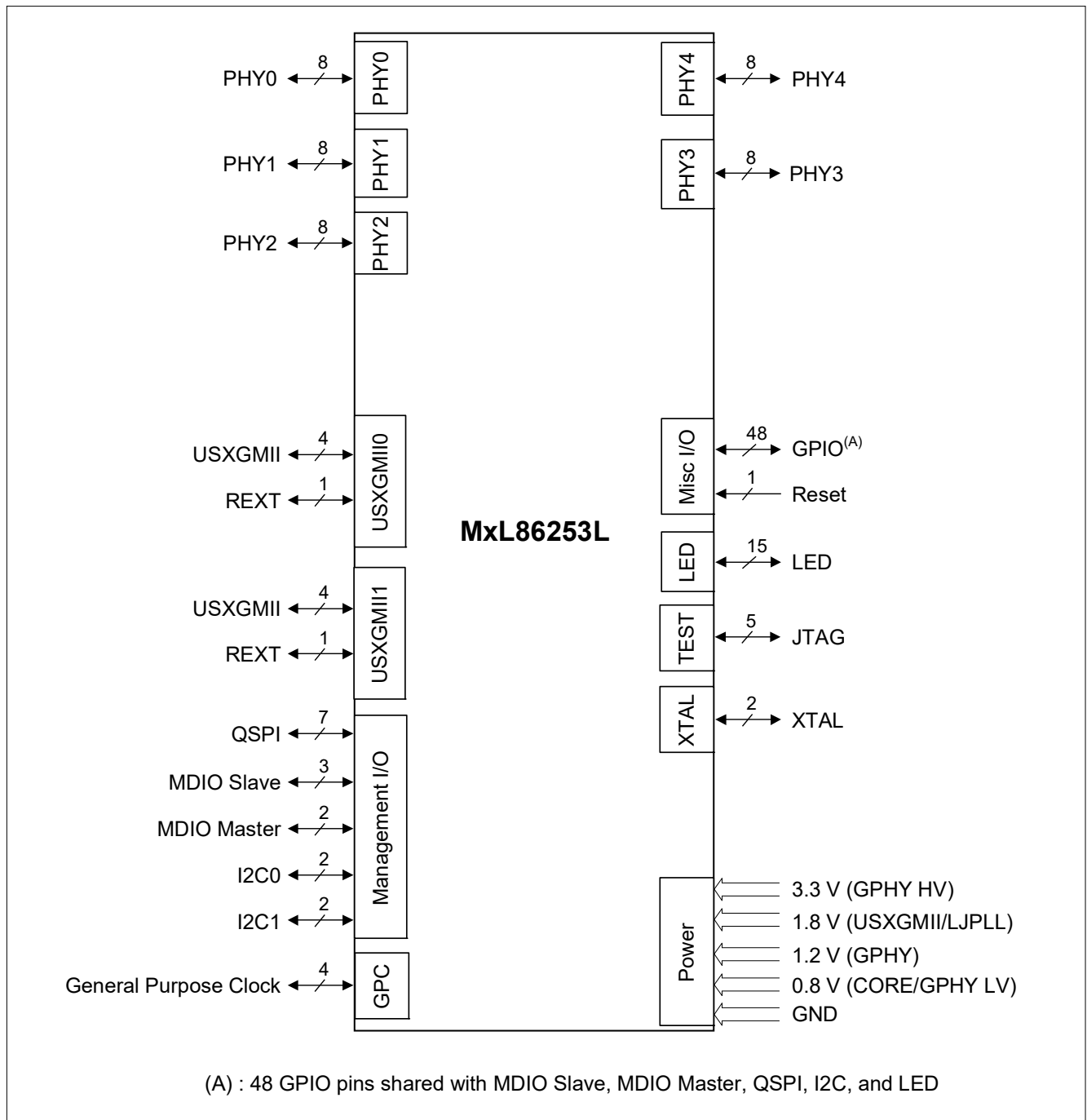
Figure 2 MxL86253L External Signal Overview
