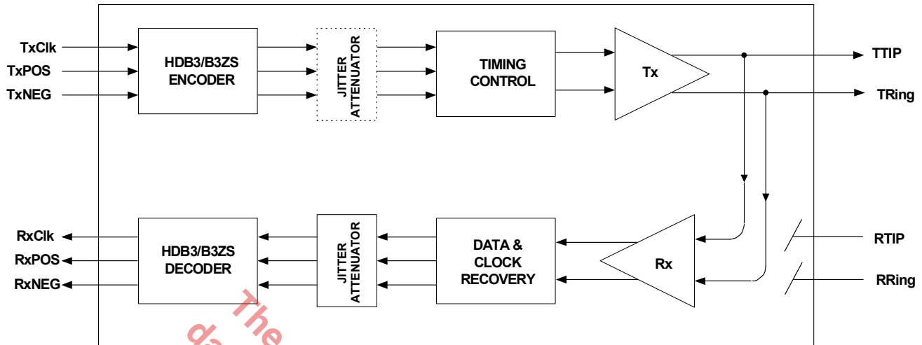
Figure 29: Analog Loopback
