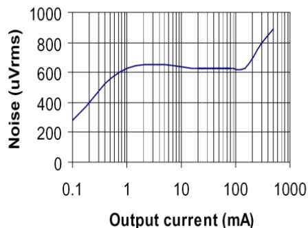
Fig. 20: Output Noise, C_{BYP} = open
