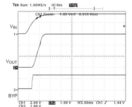
Fig. 14: Start Up Waveform, Slow V_{IN} , C_{OUT}=1000\mu F , I_O=500mA
