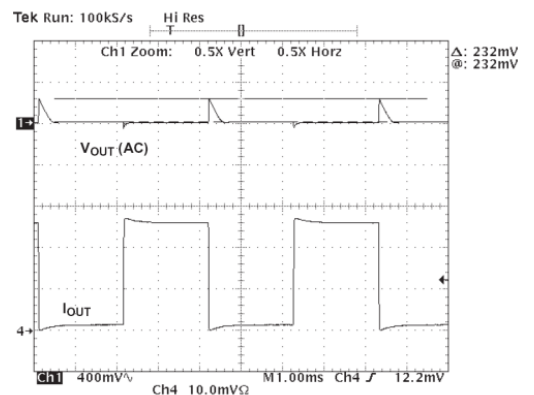
Fig. 8: Load Regulation, I_O=100\mu A \sim 500mA
