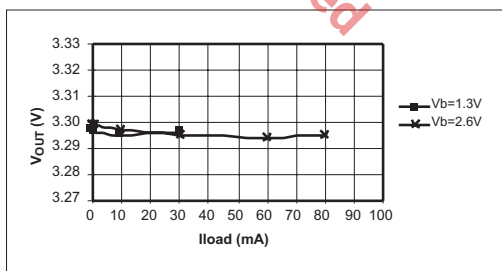
Figure 8. Line/Load Rejection vs. Output Current ( V_{out}=3.3\text{V} ), R_{lim}=5\text{k} , L_i=22\mu\text{H} Sumida CD43
