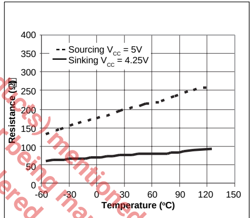
Figure 8. RESET Output Resistance vs. Temperature
