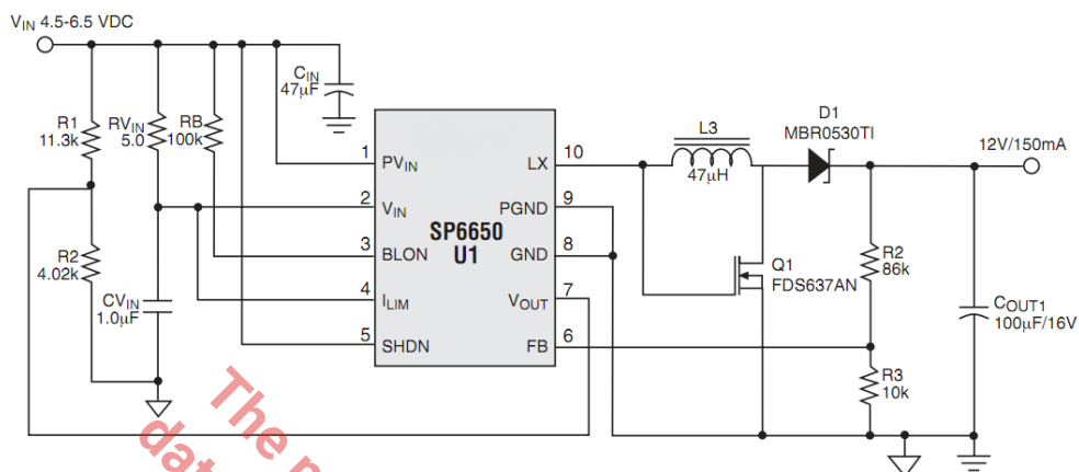
Fig.22: Additional Application Circuit: V_{IN} = 5.0V , V_{OUT} = 12V , and Max I_{LOAD} = 150mA .
