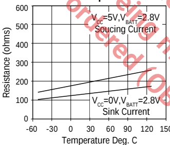
Reset Output Resistance vs. Temperature
