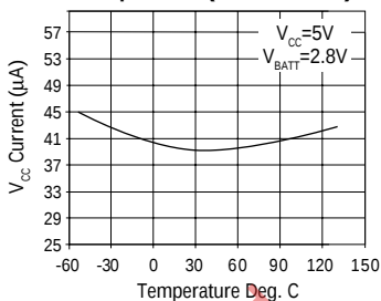
V CC Supply Current vs. Temperature (Normal Mode)
