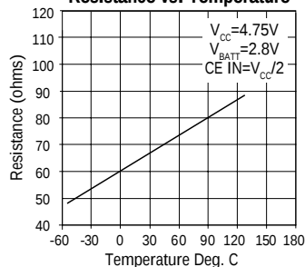
Chip Enable On Resistance vs. Temperature
