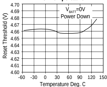
Reset Threshold vs. Temperature
