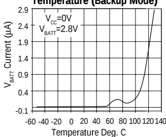
Battery Supply Current vs. Temperature (Backup Mode)
