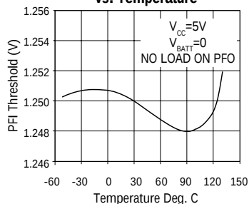
PFI Threshold vs. Temperature
