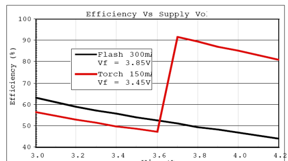
Fig. 15: Efficiency vs Supply Voltage D1=AOT3228HPW0303B LED, R_{SENSE}=0.3\Omega R_{SET}=140k\Omega , C_{IN}=2.2\mu F , C_{FC}=0.47\mu F , C_{OUT}=1\mu F
