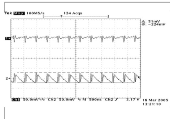
Fig. 11: Ripple 2x Torch 150mA, Ch1=VIN, Ch2=VOUT VIN=3.0V, CIN=4.7µF, CFC=0.47µF, COUT=2.2µF
