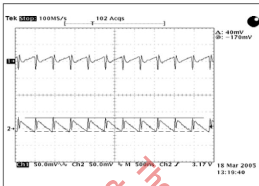
Fig. 10: Ripple 1x Torch 150mA, Ch1=VIN, Ch2=VOUT VIN=4.2V, CIN=4.7µF, CFC=0.47µF, COUT=2.2µF
