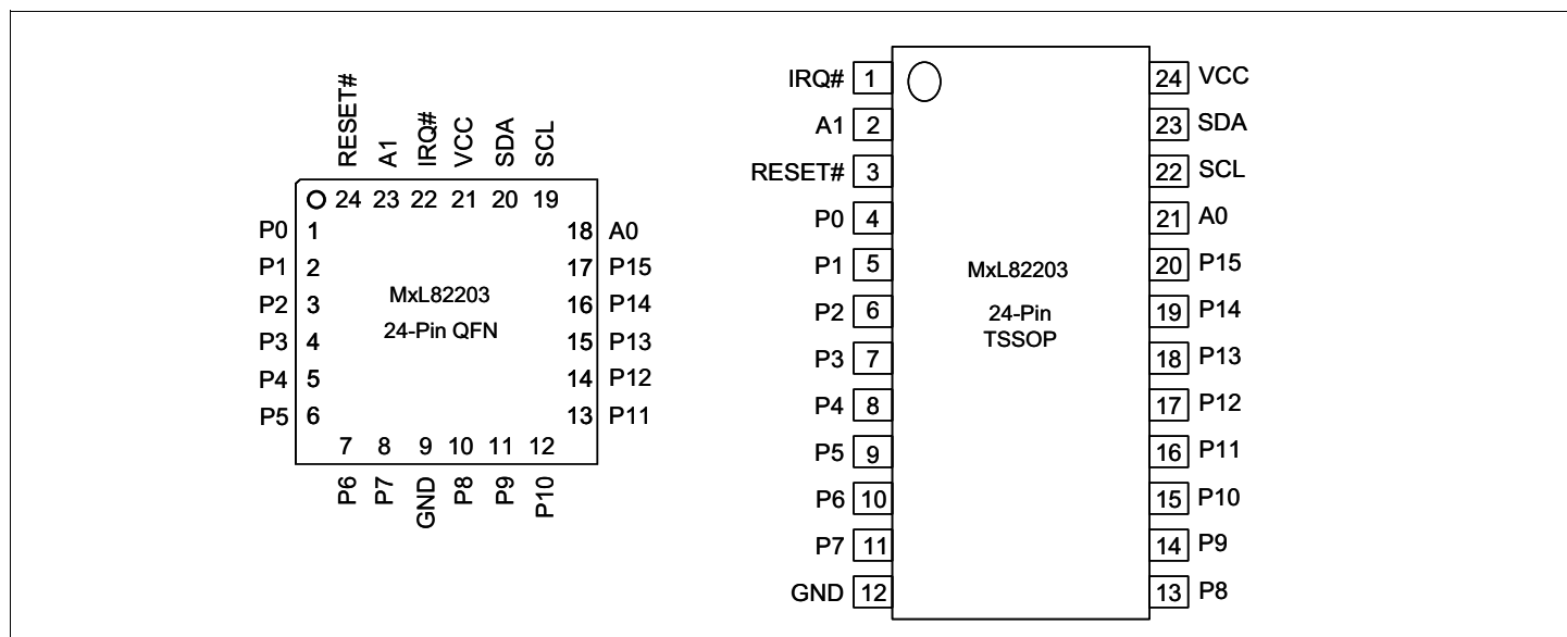
Figure 1: Pinout (Top View)
