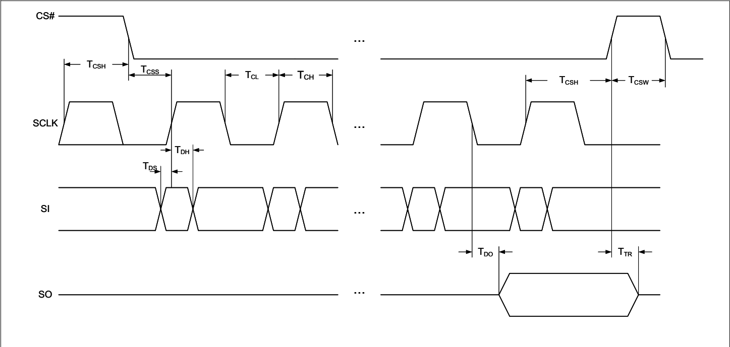
Figure 1: SPI-Bus Timing
