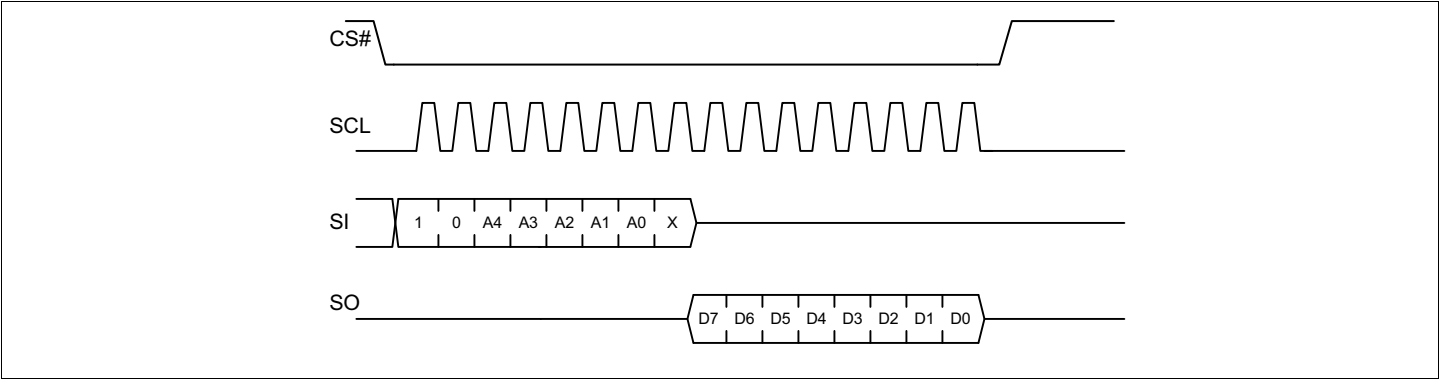
Figure 7: SPI Read
