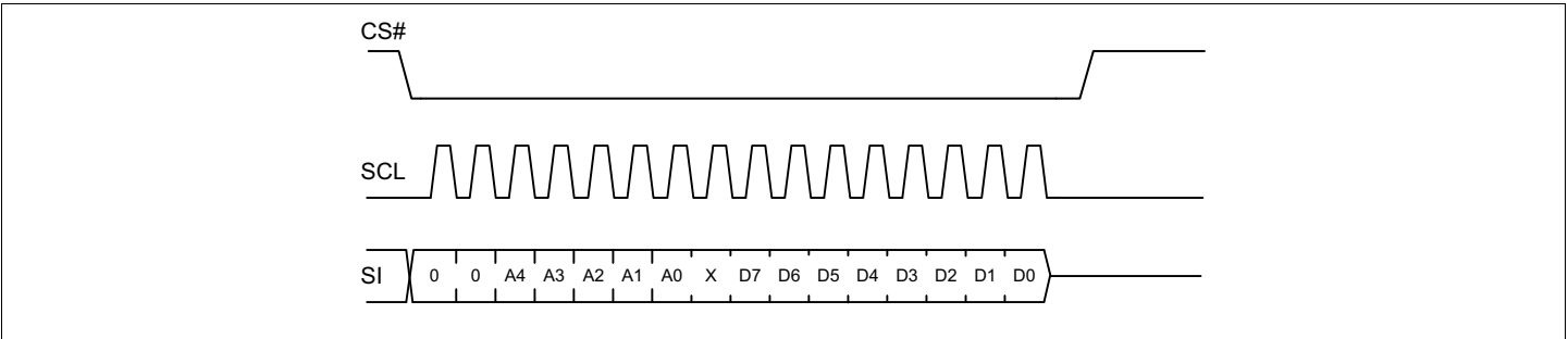
Figure 6: SPI Write
